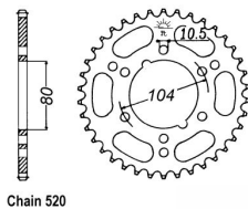
Chain 520
