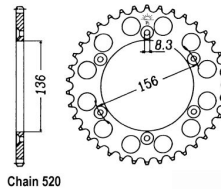
Chain 520
